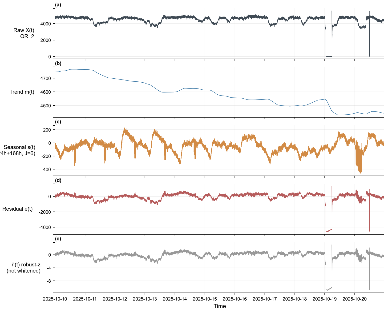
Multi-scale decomposition — QR_2 (recycle, min) [2025-10-10~2025-10-20]
